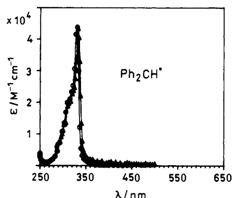
Figure 2. Absorption spectra of \text{Ph}_2\text{CH}^{\bullet} obtained on reaction (a) of e^-_{\text{solv}} with \text{Ph}_2\text{CHCl} in THF (triangles) and (b) of \text{SO}_4^{\bullet-} with \text{Ph}_2\text{CHCO}_2^- in \text{H}_2\text{O} at pH \approx 8 , [2-methyl-2-propanol] = 50 mM (circles). With b, the \epsilon scale is based on G(\text{Ph}_2\text{CH}^{\bullet}) = G(\text{SO}_4^{\bullet-}) = 3.0 .
