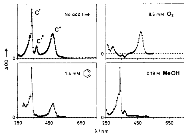
Figure 3. Effect of scavengers on the absorption spectra of the transients from bis( p -chlorophenyl)methyl chloride ( (\text{ClPh})_2\text{CHCl} ) in acetonitrile: (a) no scavenger, 70 ns after pulse; (b) oxygen saturated (8.5 mM \text{O}_2 ), 200 ns; (c) 1.4 mM 1,3-cyclohexadiene, 80 ns; (d) 0.19 M methanol, 90 ns.
